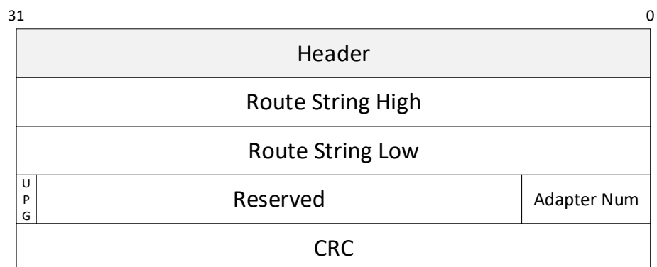
Figure 6-12. Hot Plug Event Packet
