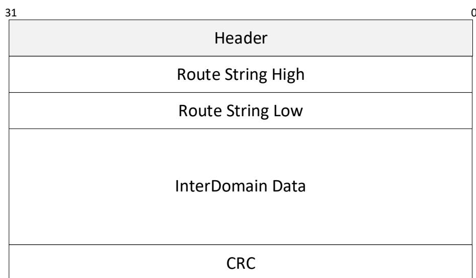
Figure 6-14. Inter-Domain Response
