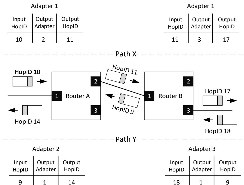
Figure 5-9. Routing Example
