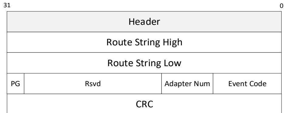
Figure 6-10. Notification Packet
