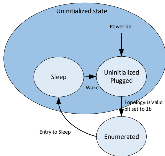
Figure 6-2. Host Router State Machine
