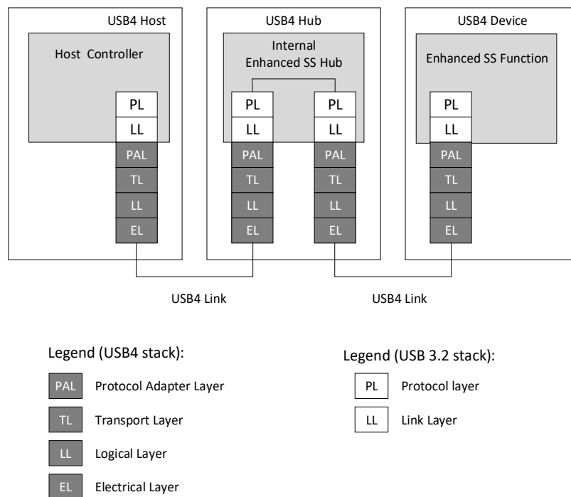
Figure 2-18. Protocol Stacks along a USB3 Tunnel
